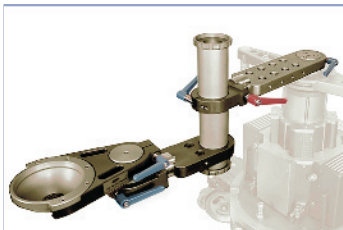
With an Off-set Ball Adapter
