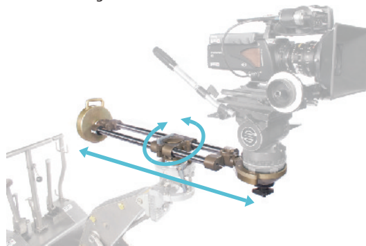
GF-Mini Bangi with standard 75cm / 2' 6" tubes, mounted on dolly
